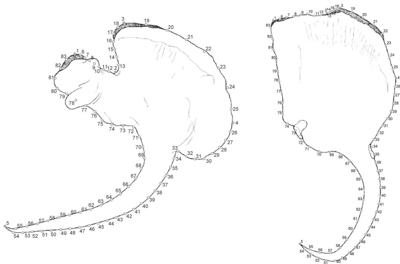
Fig. 2. Ventral and dorsal anchors of Chauhanellus boegeri Domingues and Fehlauber, 2006. Distribution of landmarks (1–5, filled points) and semi-landmarks (6–83, open points) considered in the present study in ventral and dorsal anchors. Landmarks were defined as follows: 1, top of inner root; 2, inflexion between outer root and inner root; 3, top of outer root; 4, outer shaft base; 5, tip of point. Five groups of 6–29 semi-landmarks were placed equidistantly between landmark pairs as shown.
